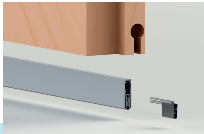
Mounting the inner profile extension
